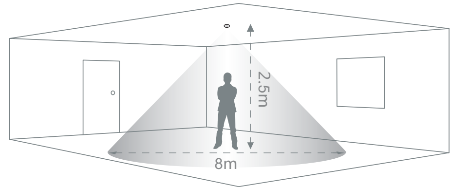
Coverage Side View
